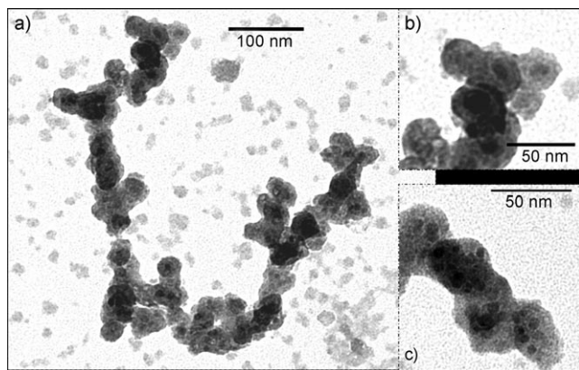
Figure 1. a) TEM images showing typical architectures of the core/shell \text{MNPs@SiO}_2(\text{RITC}) nanoparticles. b, c) Enlargements of image (a).
